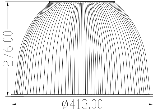
70° PC Reflector Size
